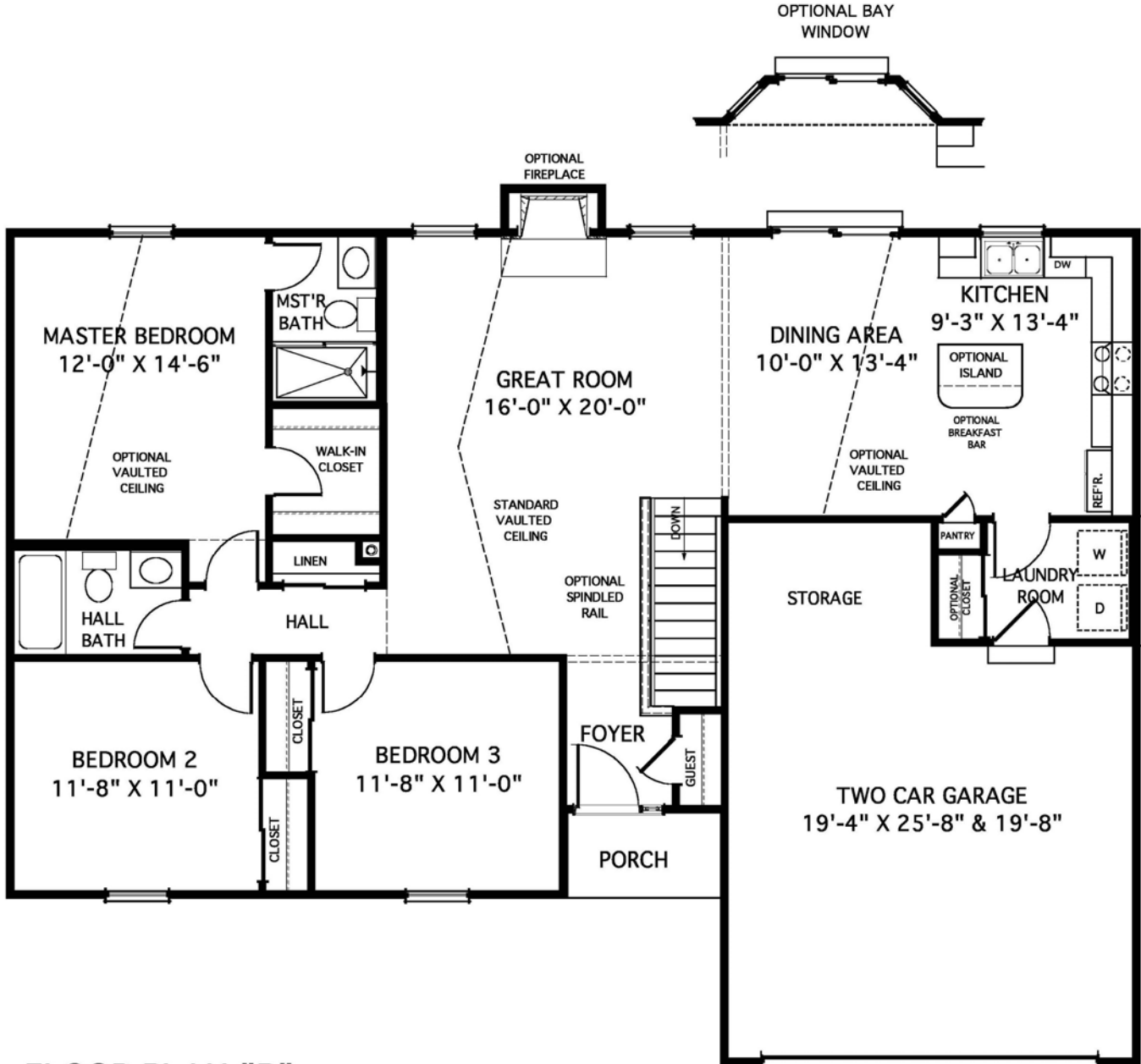
FLOOR PLAN "B"
